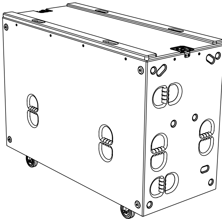
Figure 4.1 - Transport setup BSX with FDBSX
